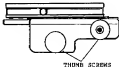
Figure 2-19. ART II mount.
